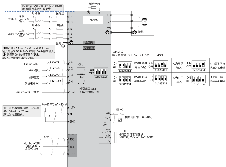
图9-16 三相/单相电源输入 (MD600S-4T1R6~ MD600S-4T9R5B, MD600S-2S2R8~ MD600S-2S010B) 端子接线图
